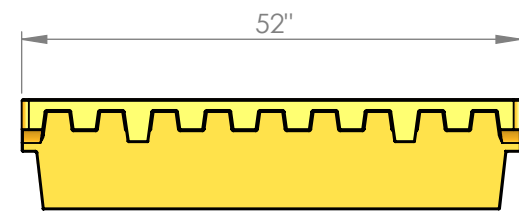
RIGHT VIEW
